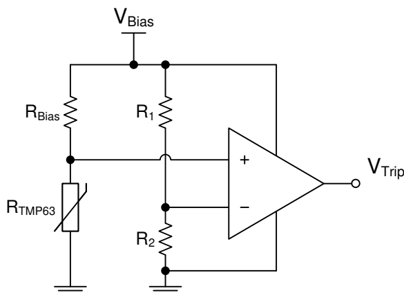
Figure 18. Temperature Switch Using Voltage Divider and a Comparator
