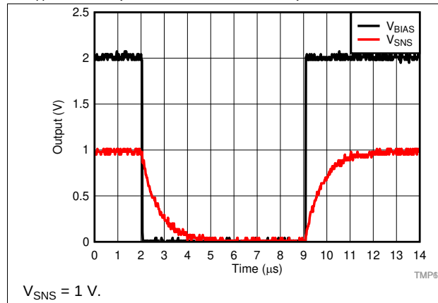
Figure 7. Step Response
