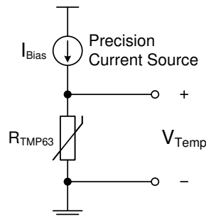
Figure 16. Biasing Circuit With Current Source
