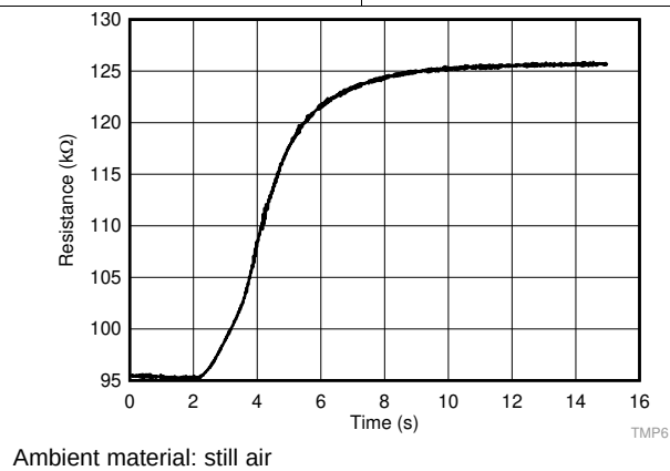
Figure 9. Thermal Response Time
