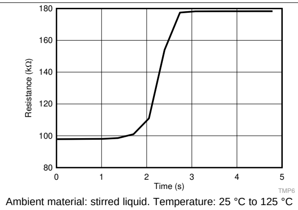
Figure 8. Thermal Response Time
