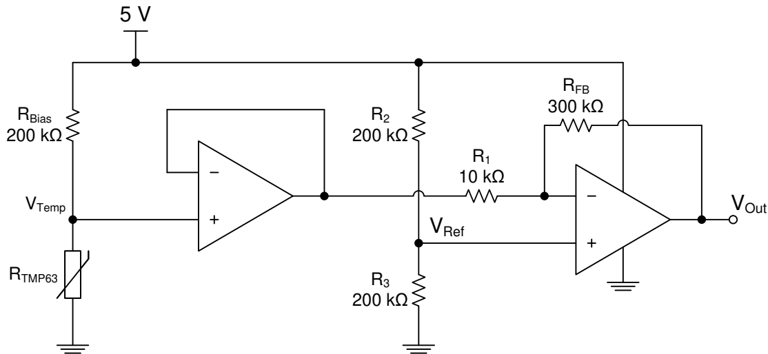
Figure 19. Thermal Foldback Using Voltage Divider and a Rail-to-Rail Op Amp
