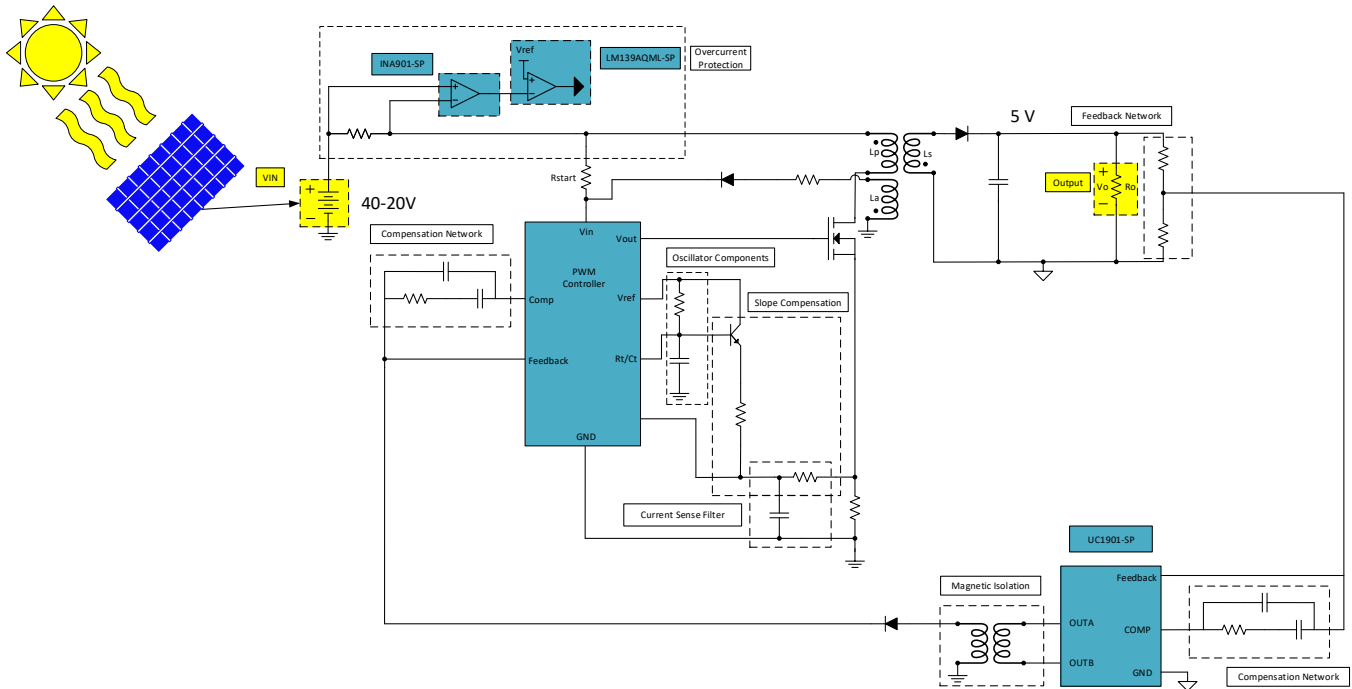
Figure 1. Test Setup
