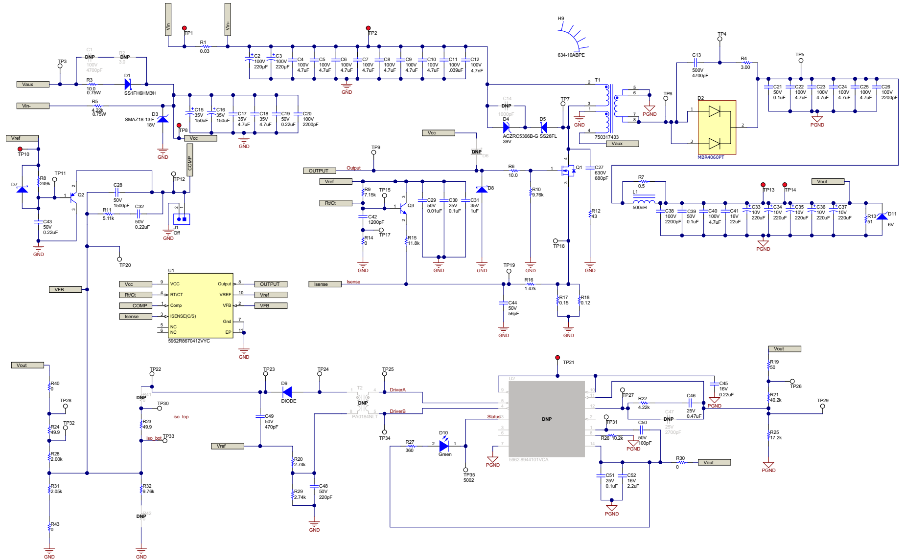
Figure 31. UC1843BEVM-CVAL Schematic 01
