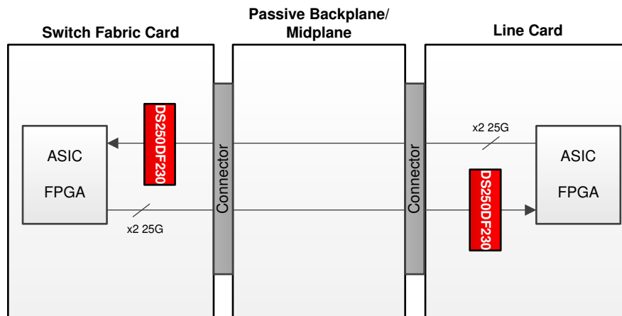
Figure 24. Backplane/Mid-Plane Application Block Diagram
