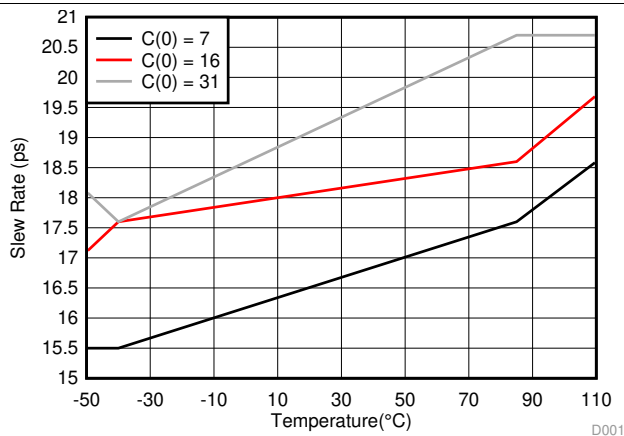
Figure 1. Output Transition-time vs Ambient Temperature
