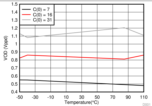
Figure 2. Typical VOD vs Ambient Temperature
