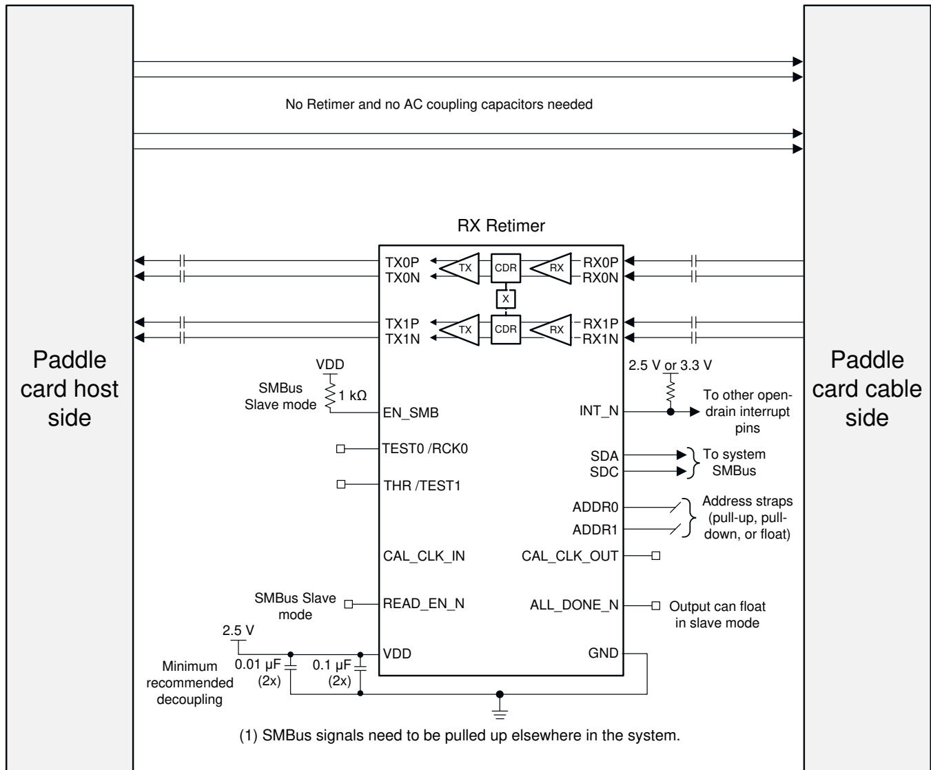
Figure 22. Half-Active Cable Application Schematic
