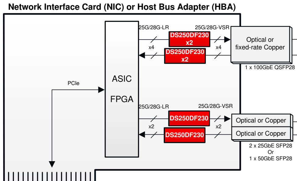
Figure 17. Front-Port Application Block Diagram
