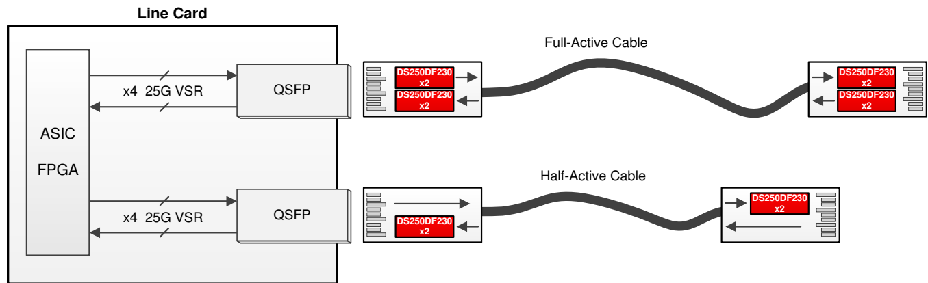
Figure 21. Active Cable Application Block Diagram
