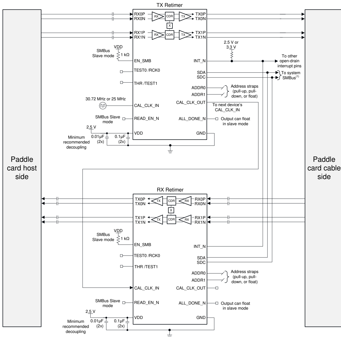
Figure 23. Full-Active Cable Application Schematic
