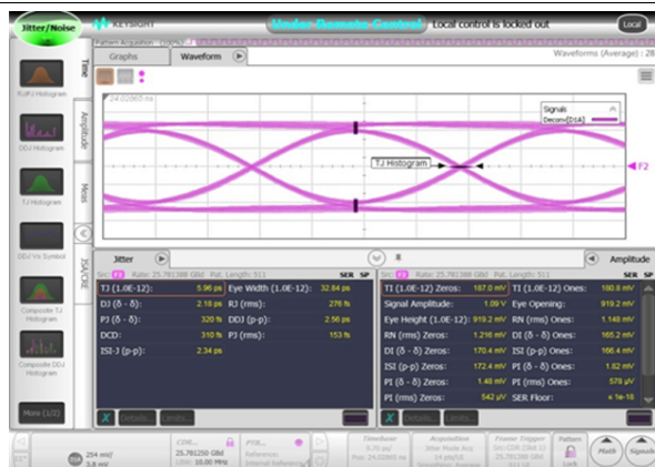
Figure 19. DS250DF230 Operating at 25.78125 Gbps
