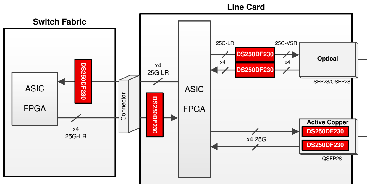
Figure 15. Typical Uses for the DS250DF230 in a System
