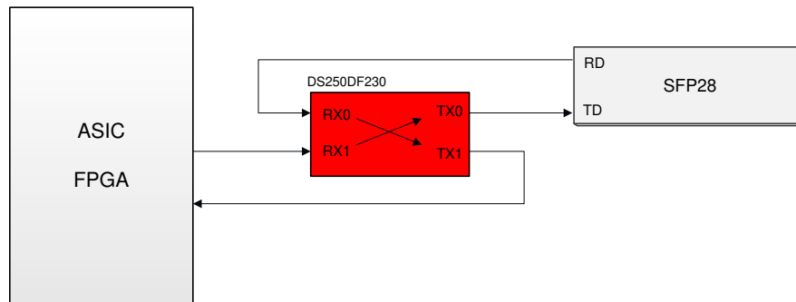
Figure 16. Bidirectional Application
