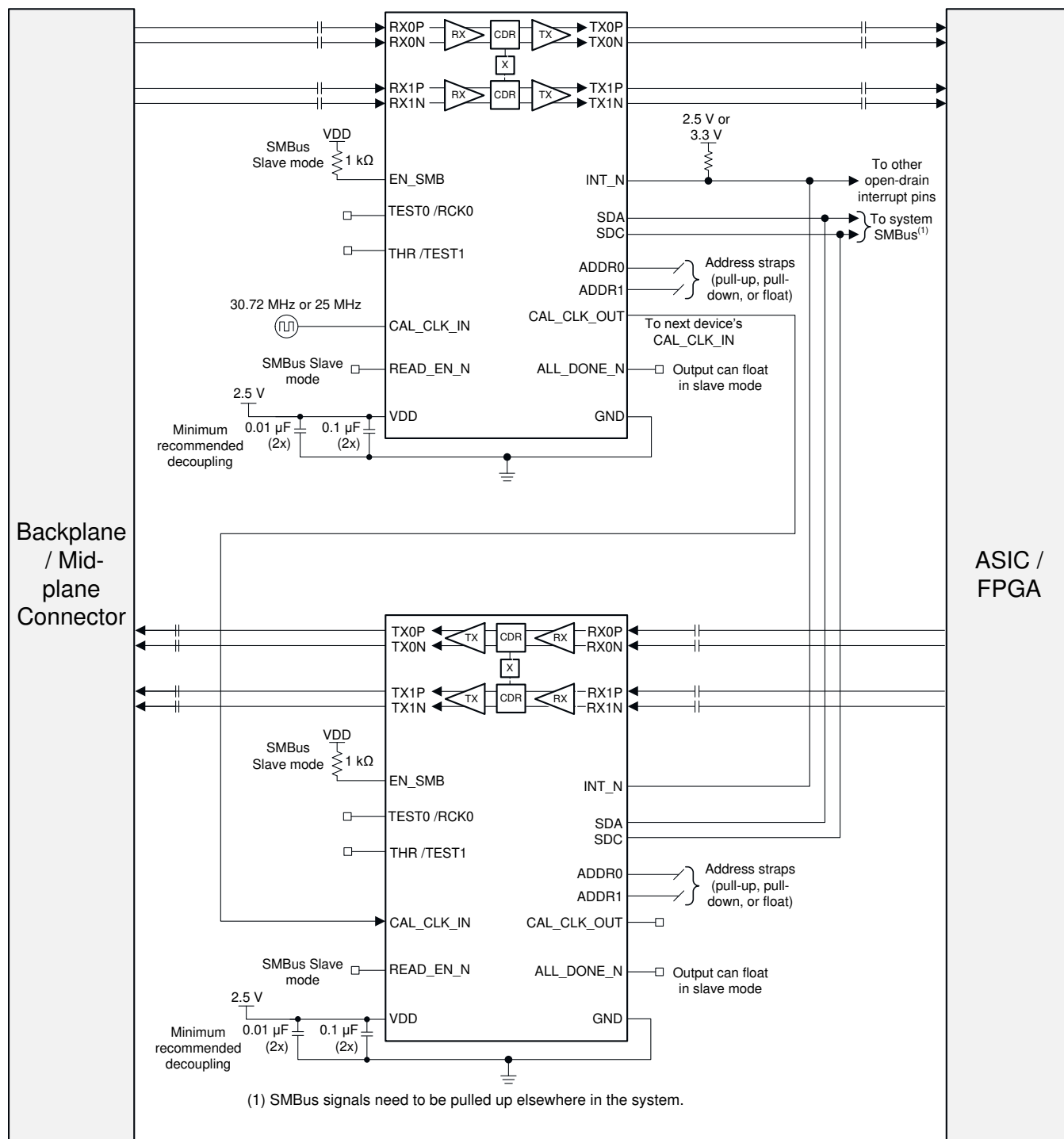
Figure 25. Backplane/Mid-Plane Application Schematic
