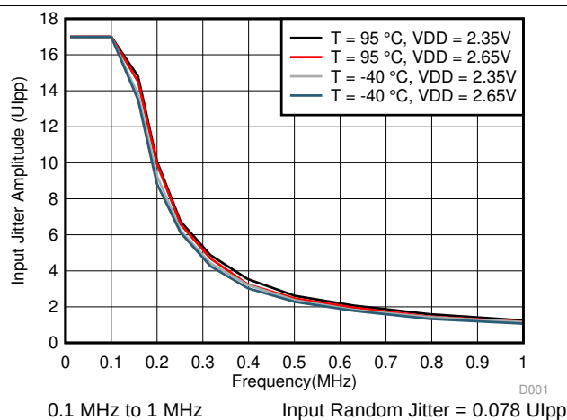
Figure 5. Typical Sinusoidal Input Jitter Tolerance for 30-dB Channel at 25.78125 Gbps
