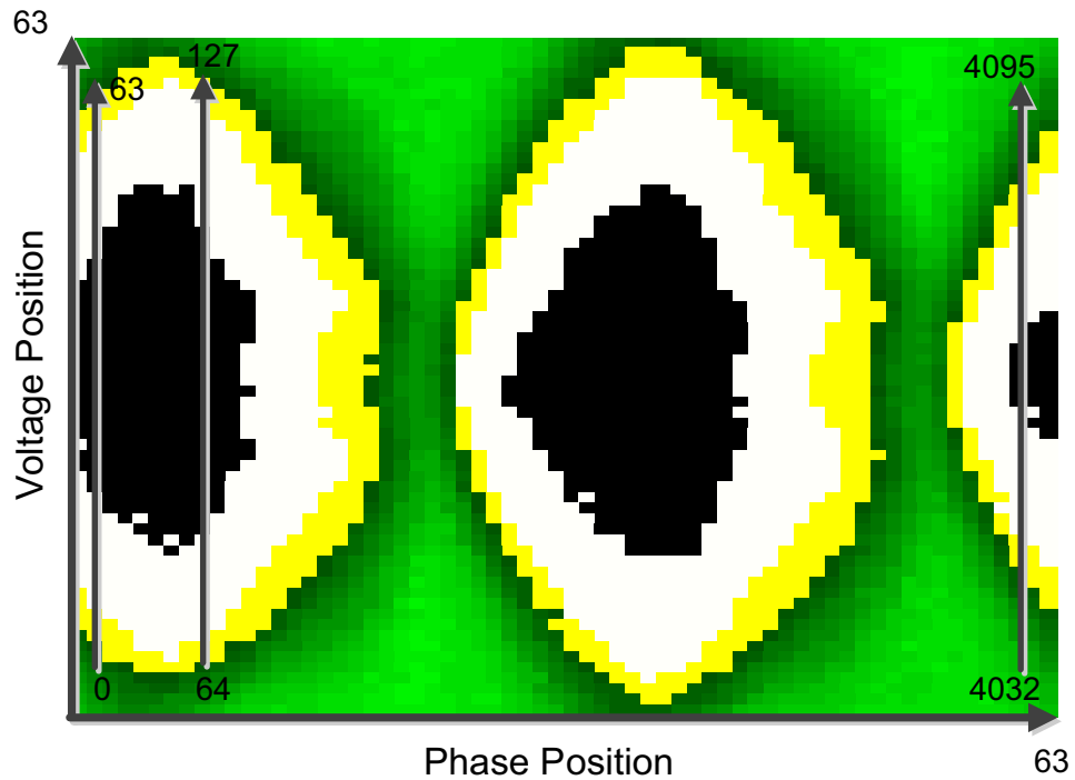
Figure 14. EOM Full Eye Capture Readout
