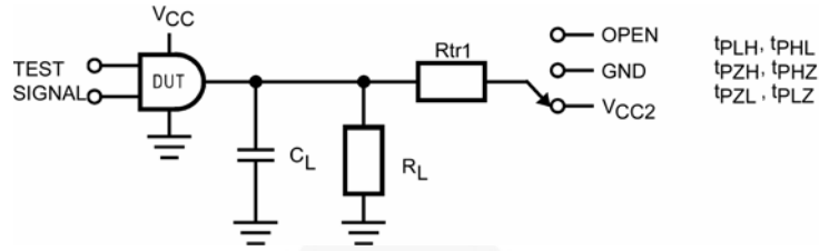
Figure 2. AC Test Circuit
