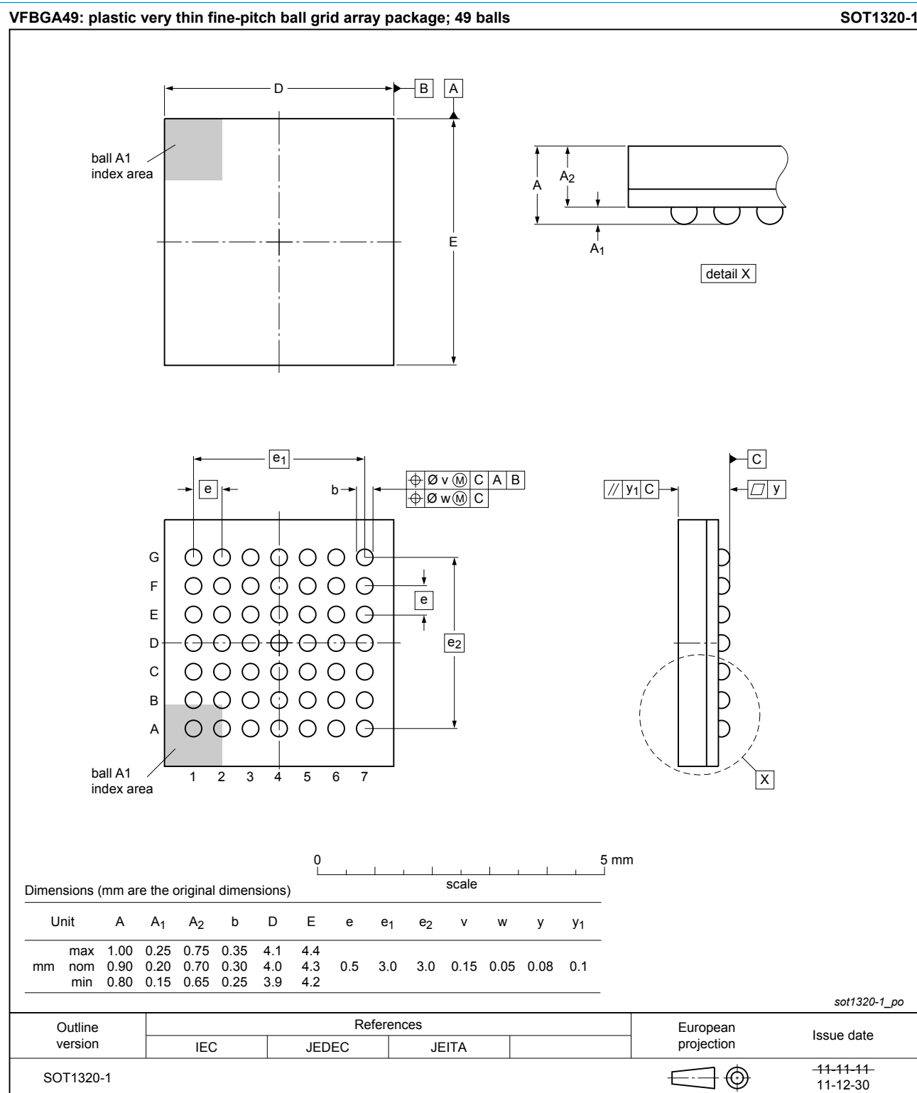
Figure 29. Package outline, VFBGA49, SOT1320-1, MSL 1
