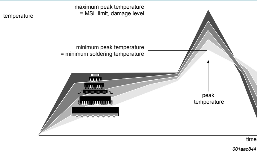
Figure 30. Temperature profiles for large and small components
