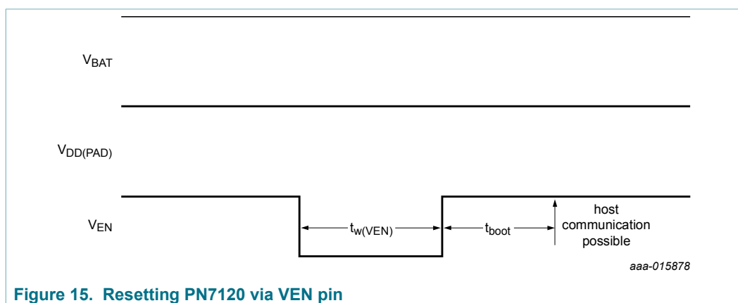
Figure 15. Resetting PN7120 via VEN pin
