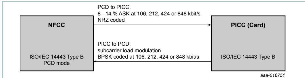
Figure 22. ISO/IEC 14443B Reader/Writer communication mode diagram
