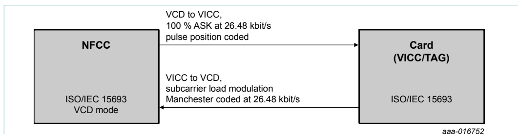
Figure 23. R/W mode for NFC forum T5T communication diagram
