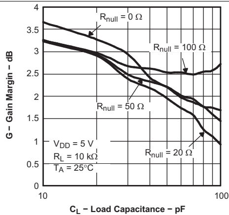
Figure 21. Gain Margin vs Load Capacitance
