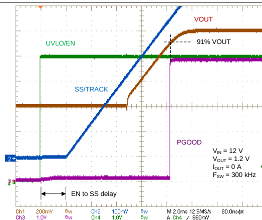
Figure 18. Prebias Start-up Characteristic
