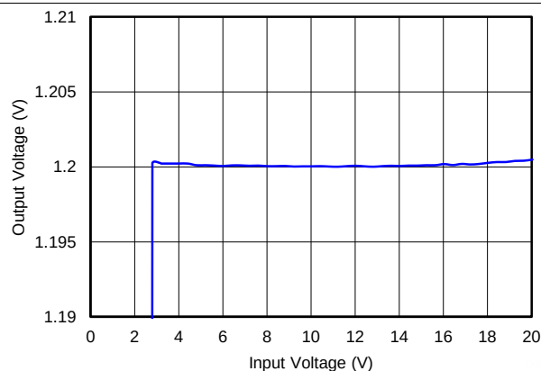
Figure 4. Line Regulation
