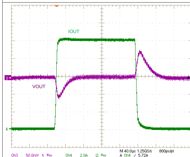
Figure 44. Load Transient Response at V_{OUT} = 1.2 V, I_{OUT} 0A to 10A at 2A/ \mu s
