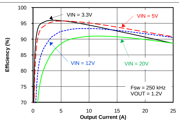
Figure 43. Efficiency vs. Output Current at V_{OUT} = 1.2 V
