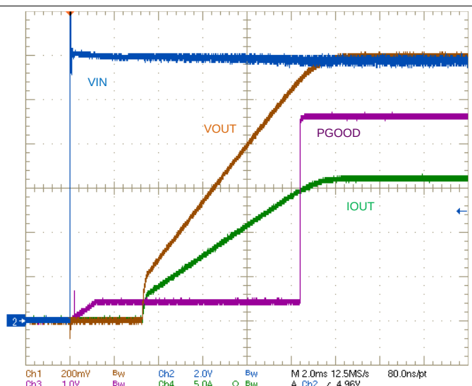
Figure 45. Startup Characteristic with V_{IN} stepped from 0 V to 12 V, V_{OUT} = 1.2 V, 70-m \Omega Load
