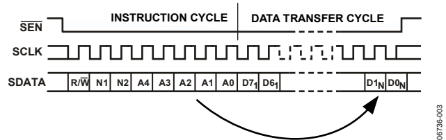
Figure 3. SPI Timing, MSB First
