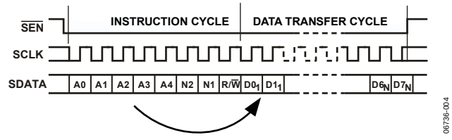
Figure 4. SPI Timing, LSB First
