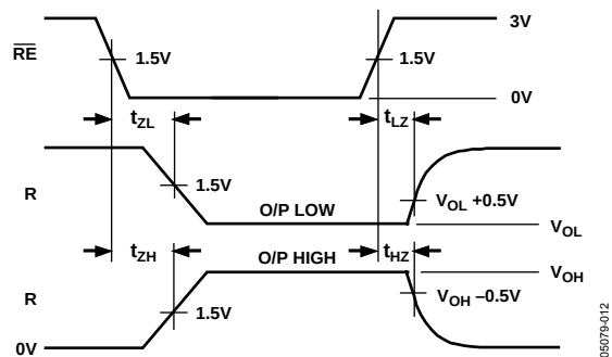
Figure 12. Receiver Enable/Disable Timing
