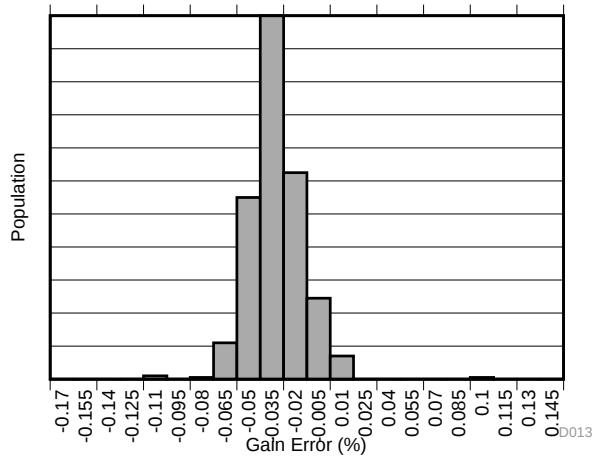
Figure 13. Gain Error Production Distribution A3
