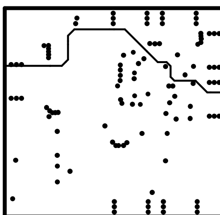
Figure 6-5. Power Layer
