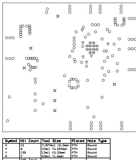
Figure 6-9. Drill Drawing
