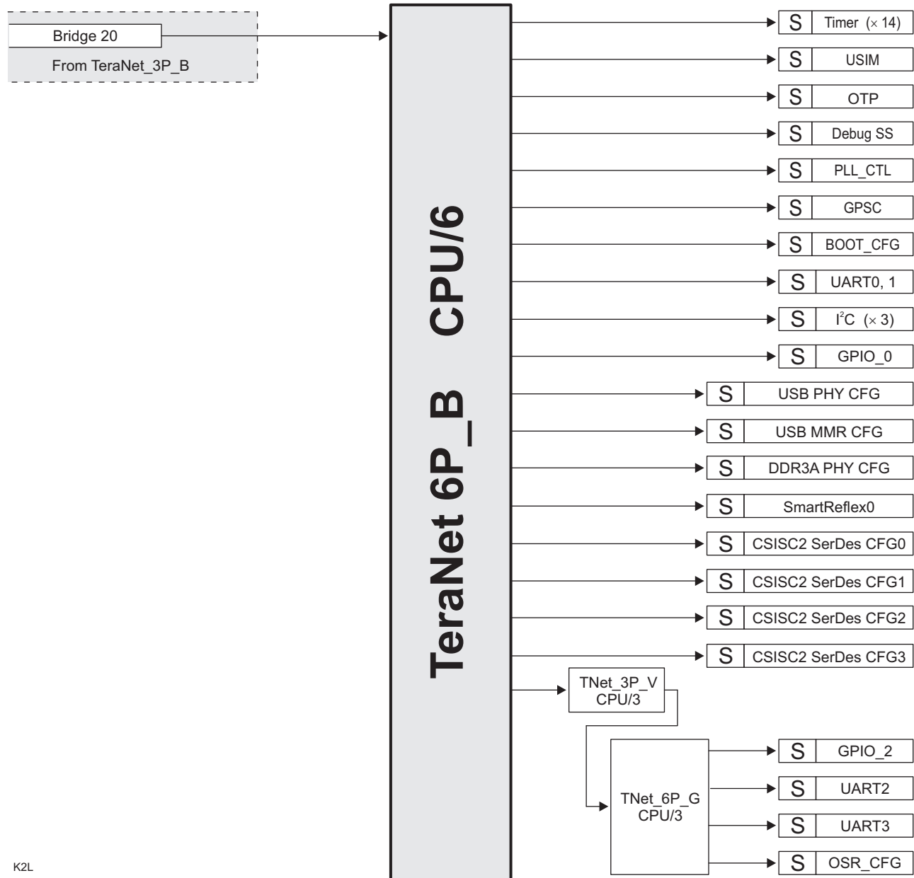
Figure 8-8. TeraNet 6P_B
