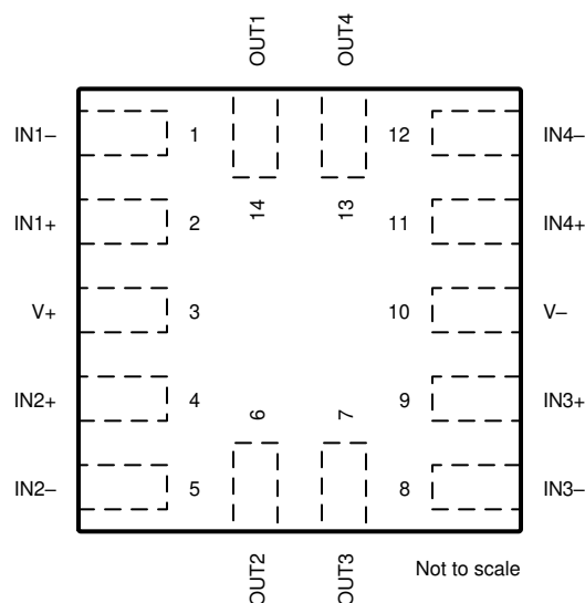
OPA4990 RUC Packages (1) 14-Pin X2QFN With Exposed Thermal Pad Top View
