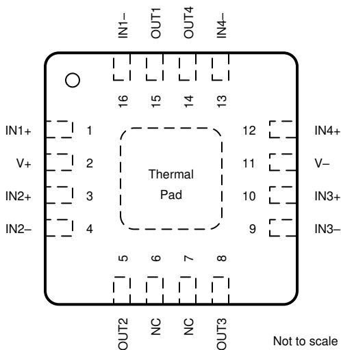
OPA4990 RTE Package (1)(2) 16-Pin WQFN With Exposed Thermal Pad Top View
