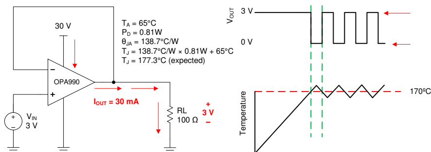
Figure 51. Thermal Protection
