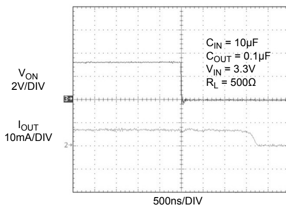
Figure 16. t_{d_{OFF}} Response
