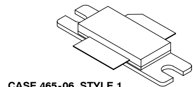
CASE 465-06, STYLE 1 NI-780 MRF19085LR3
