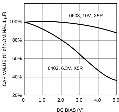
Figure 19. Typical Variation in Capacitance vs. DC Bias
