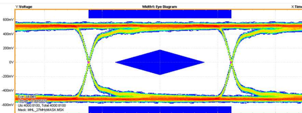
Figure 13. Eye Pattern: 0.7-Gbps MHL Eye Pattern for With No Device
