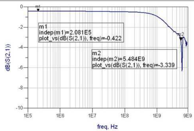
Figure 4. Gain vs Frequency for MHL Switch
