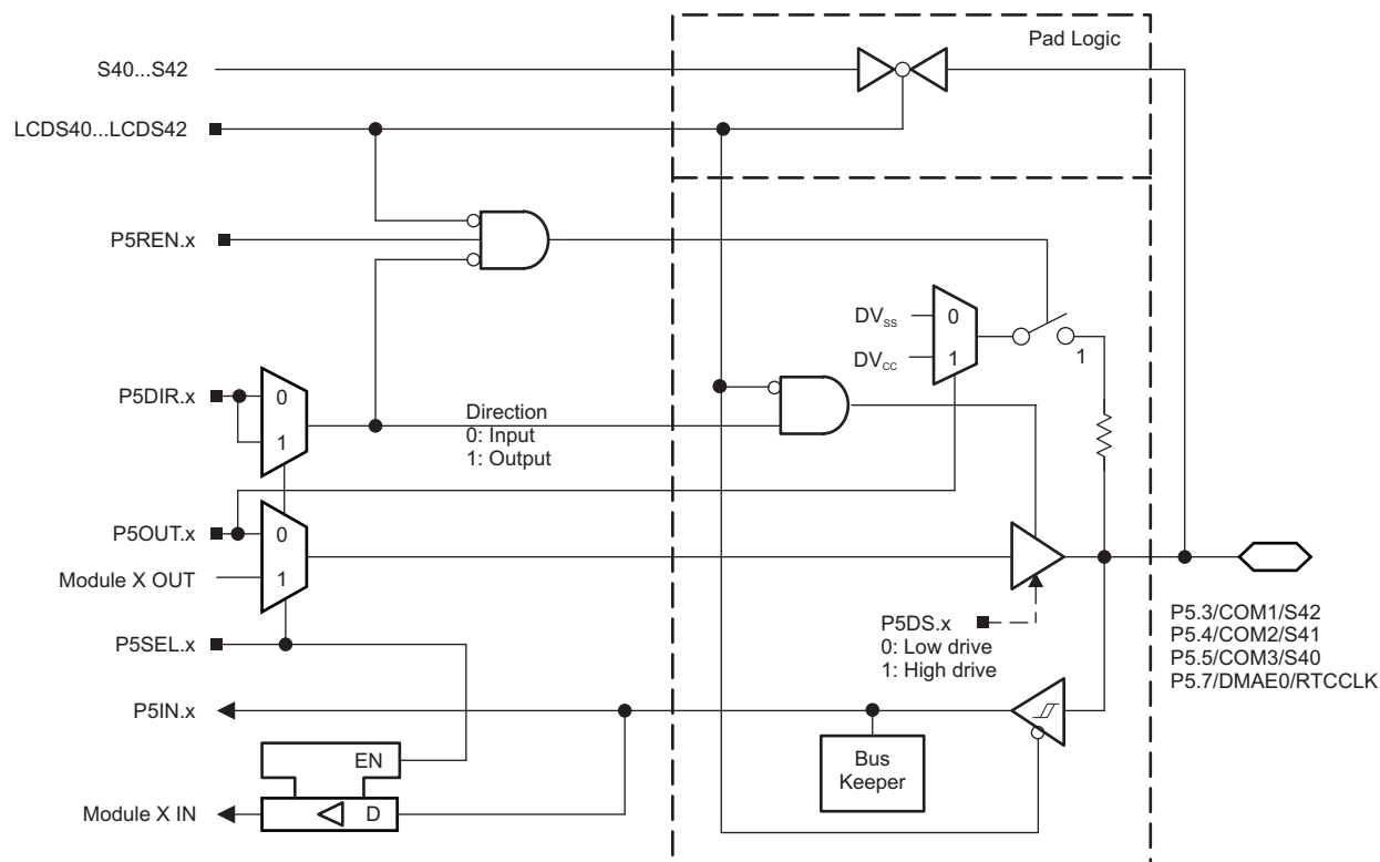
Figure 6-9. Port P5 (P5.3 to P5.5 and P5.7) Diagram
