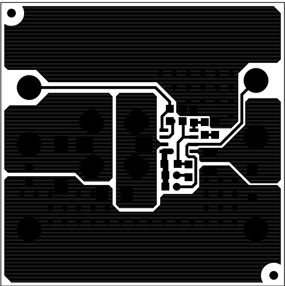
Component Side
