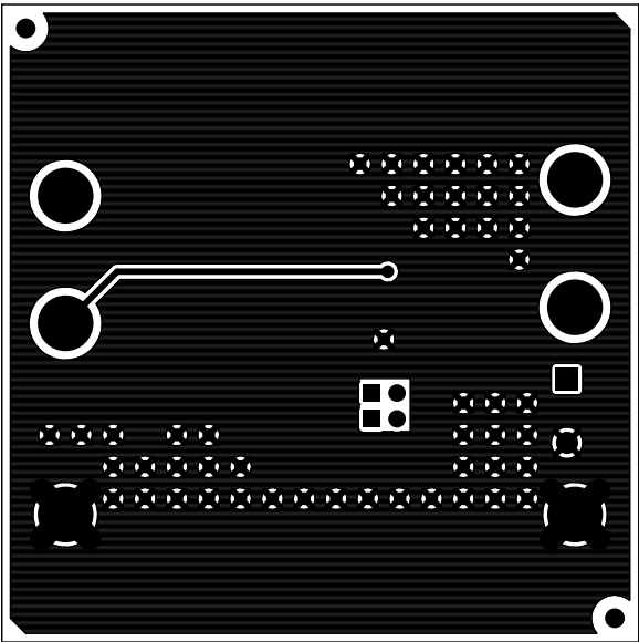
Solder Side
