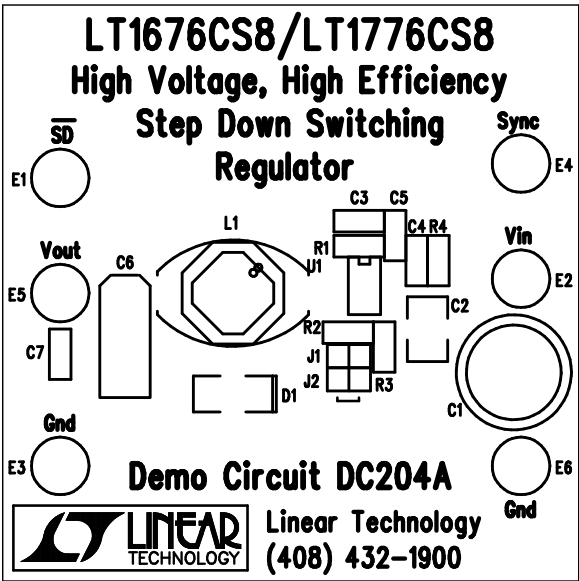
Silkscreen Top
