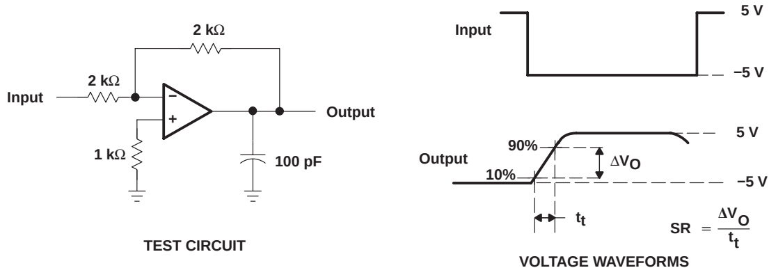
Figure 1. Slew Rate
