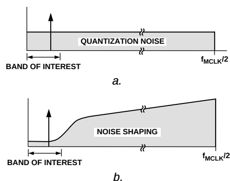
Figure 21. Sigma-Delta ADC
