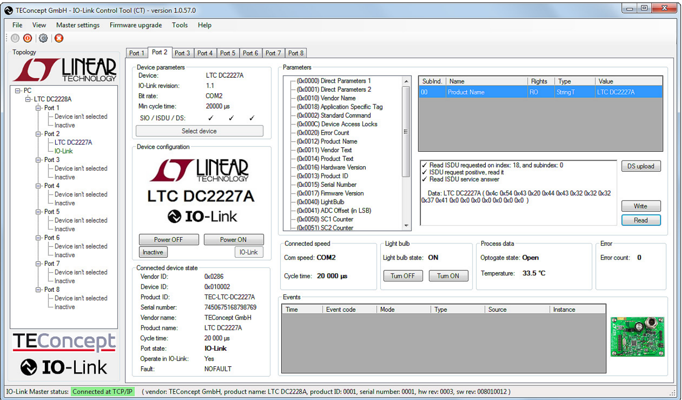
Figure 2. Control Tool for Connecting DC2227A to DC2228A
