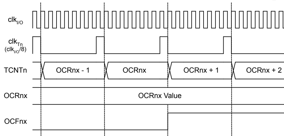
Figure 21-10. Timer/Counter Timing Diagram, Setting of OCF1x, with Prescaler ( f_{\text{clk}_{I/O}/8} )
