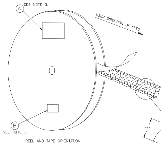
REEL AND TAPE ORIENTATION
