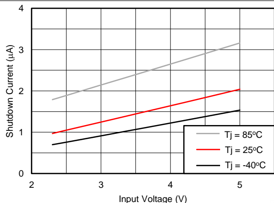
Figure 7. Shutdown Current vs Input Voltage (Boost Mode)
