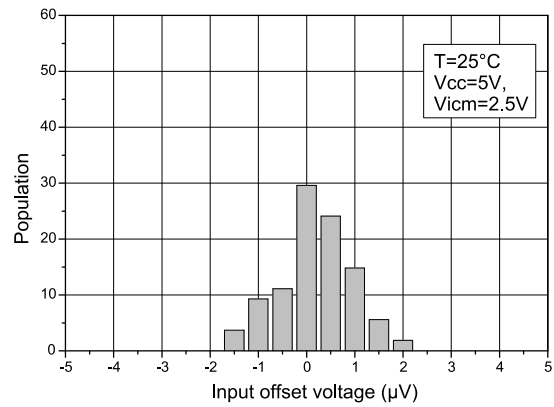
Figure 3: Input offset voltage distribution at VCC = 5 V
