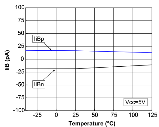
Figure 19: Input bias current vs. temperature at VCC = 5 V
