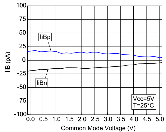
Figure 17: Input bias current vs. common mode at VCC = 5 V
