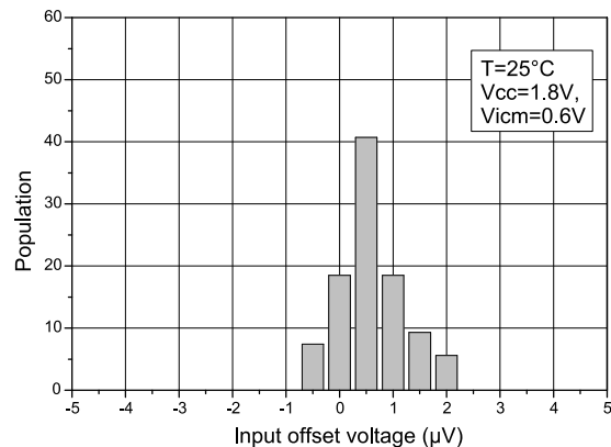
Figure 5: Input offset voltage distribution at VCC = 1.8 V
