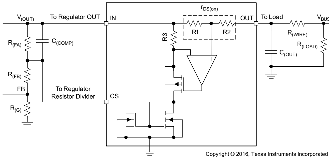
Figure 38. Cable Compensation Equivalent Circuit
