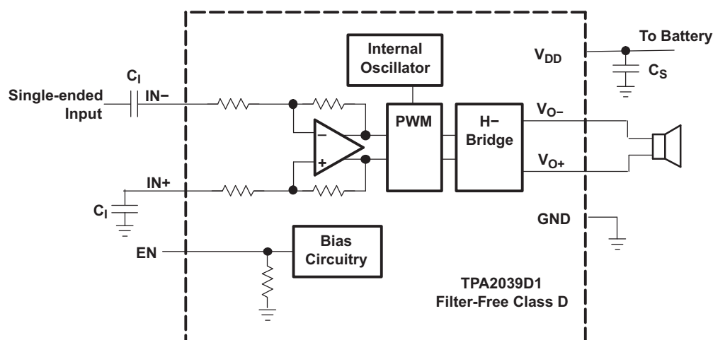
Figure 30. TPA2039D1 Application Schematic With Single-Ended Input
