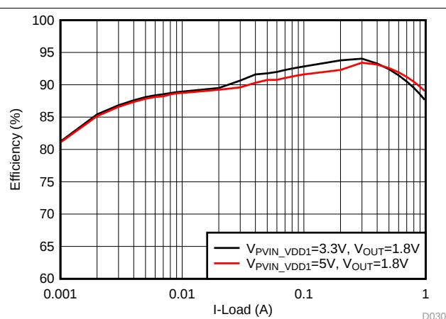
Figure 34. VDD1 Efficiency Curve, V_{OUT} = 1.8 V
