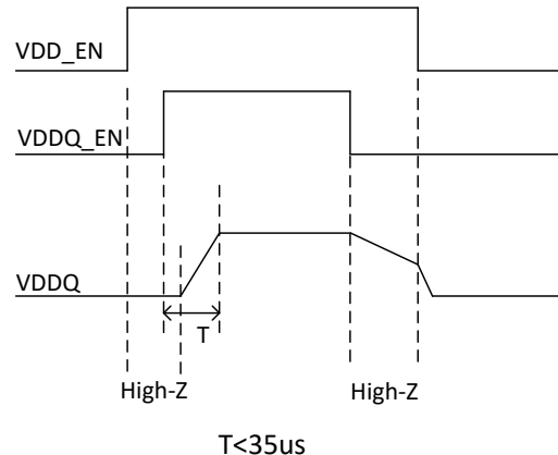
Figure 30. Power Sequence, VDDQ vs VDDQ_EN
