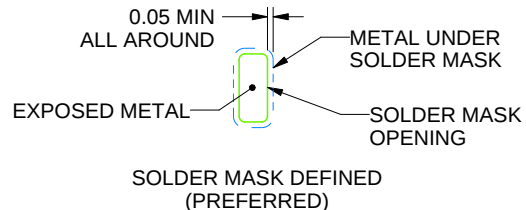
SOLDER MASK DETAILS
