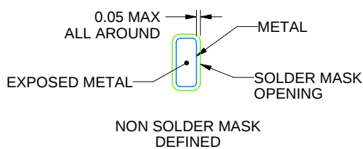
SOLDER MASK DETAILS
