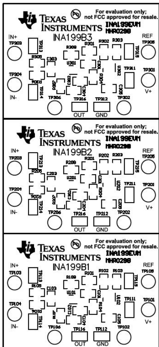
Figure 2. INA199EVM Top Overlay
