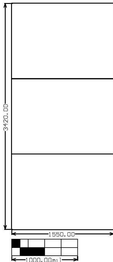
Figure 8. INA199EVM Board Dimensions
