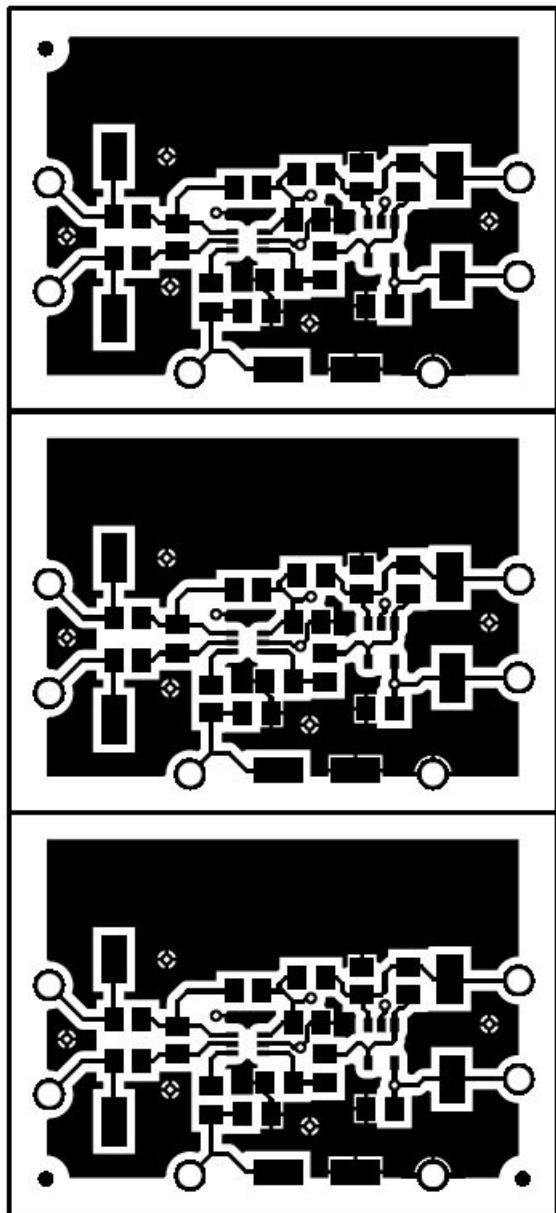
Figure 4. INA199EVM Top Layer
