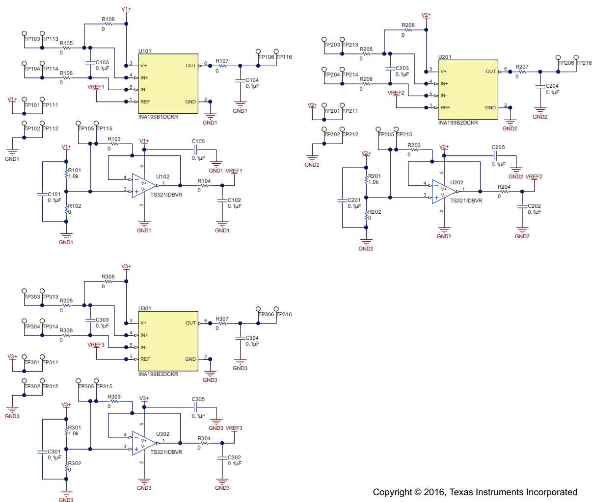
Figure 1. INA199EVM Schematic
