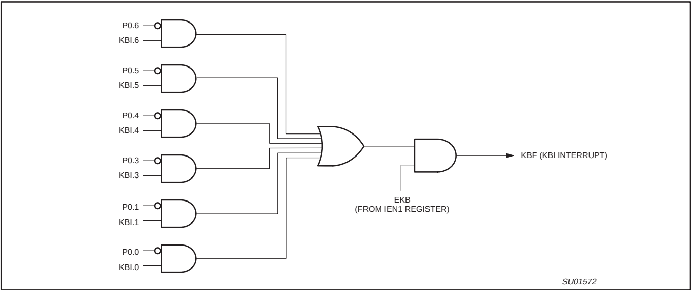
Figure 14. Keyboard Interrupt
