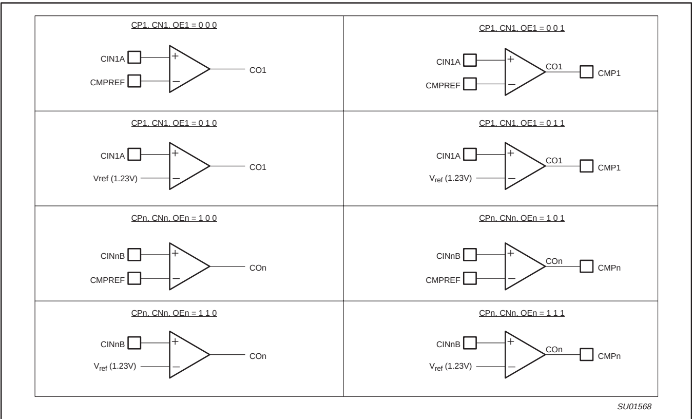
Figure 4. Comparator Configurations
