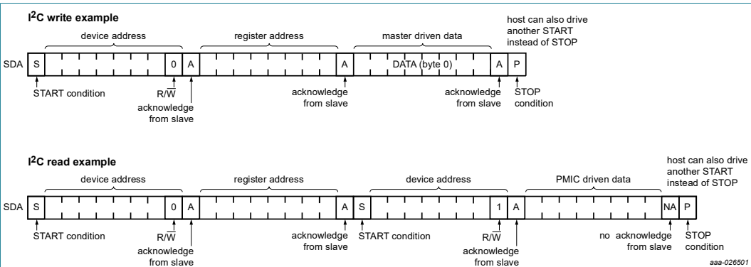
Figure 13. I 2 C sequence
