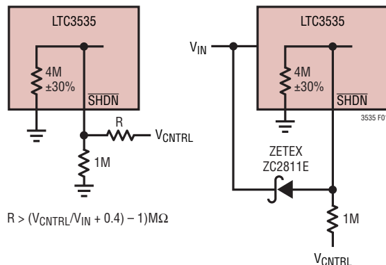
Figure 1. Recommended Shutdown Circuits When Driving SHDN Above V_{IN}
