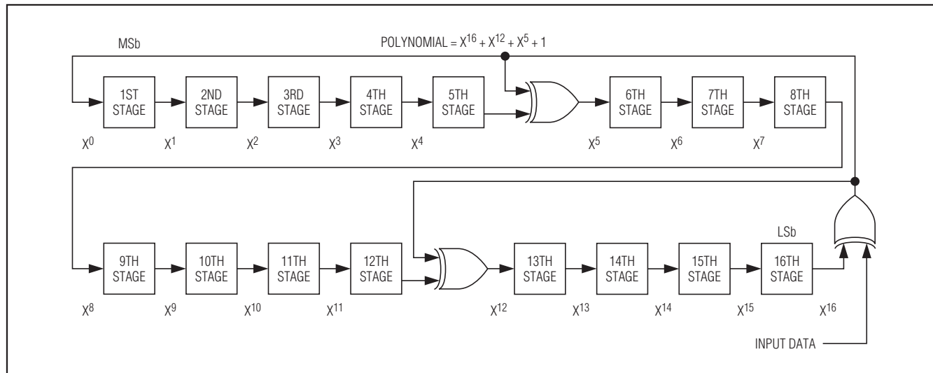
Figure 32. CRC-16-CCITT Generator
