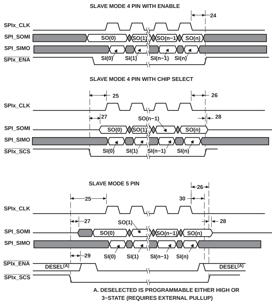
Figure 4-36. SPI Timings—Slave Mode (4-Pin and 5-Pin)
