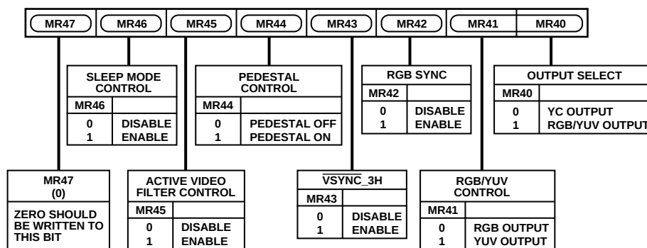
Figure 42. Mode Register 4
