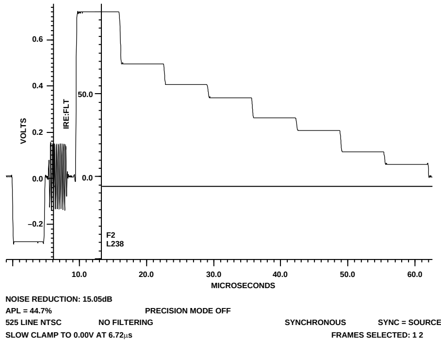
Figure 87. 100/7.5/75/7.5 NTSC Color Bars Luminance
