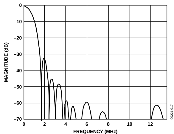
Figure 17. CIF Chroma Filter
