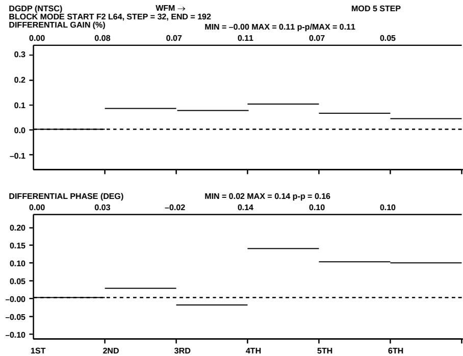
Figure 92. NTSC Differential Gain and Phase Measurement
