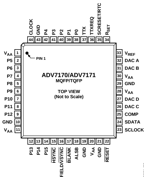
Figure 5. Pin Configuration
