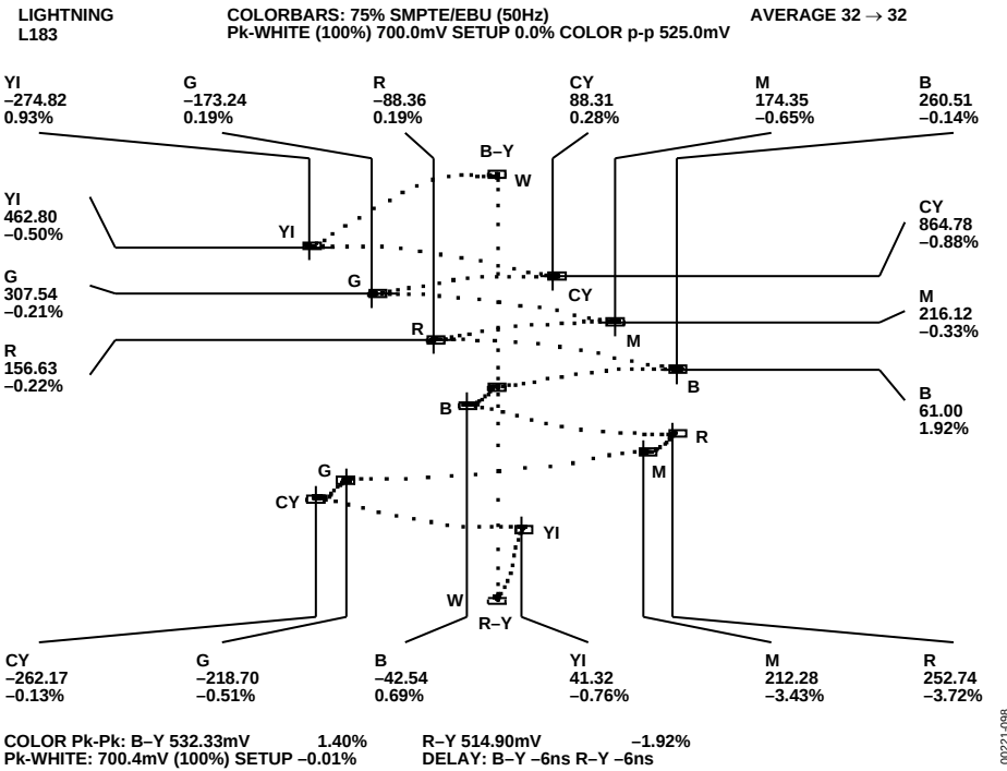
Figure 98. PAL YUV Lighting Plot
