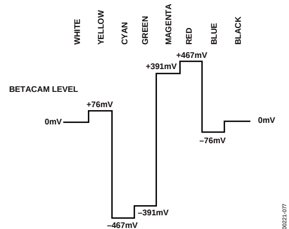
Figure 76. NTSC 100% Color Bars, No Pedestal V Levels
