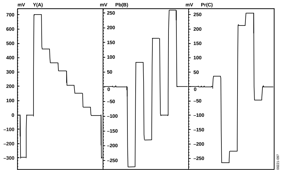
Figure 97. PAL YUV Parade Plot
