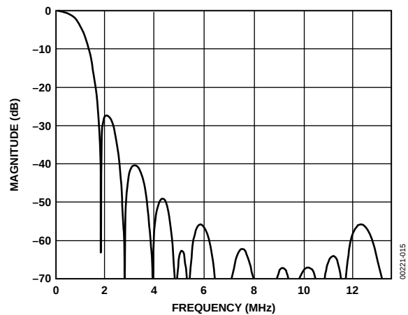
Figure 15. 1.0 MHz Low-Pass Chroma Filter
