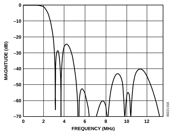
Figure 16. 2.0 MHz Low-Pass Chroma Filter
