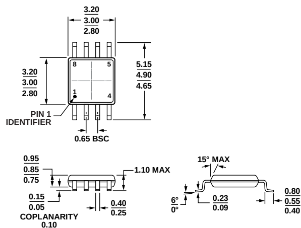
COMPLIANT TO JEDEC STANDARDS MO-187-AA Figure 66. 8-Lead Mini Small Outline Package [MSOP] (RM-8)
