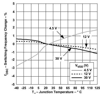
Figure 10. Switching Frequency Change vs Junction Temperature
