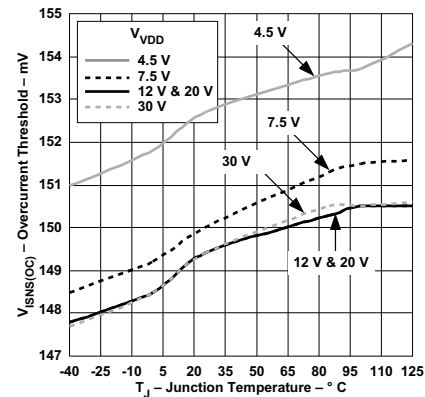
Figure 8. Overcurrent Threshold vs Junction Temperature
