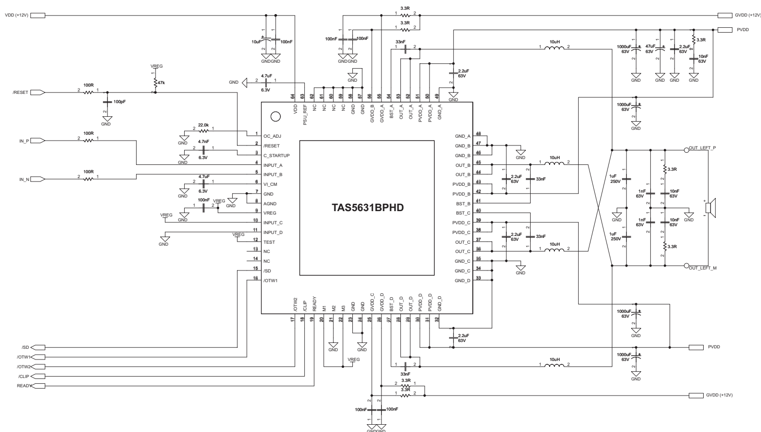
Figure 15. Typical Differential (2N) BTL Application With BD Modulation Filters
