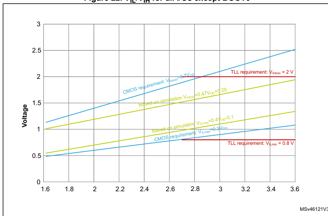
Figure 22. V_{IL}/V_{IH} for all I/Os except BOOT0
