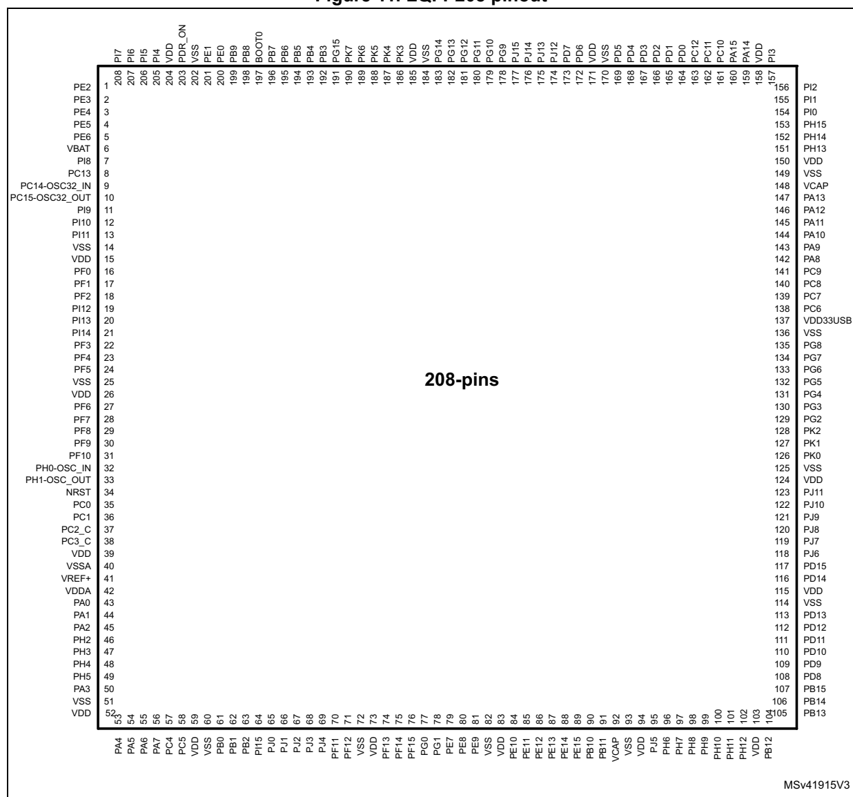
Figure 11. LQFP208 pinout
