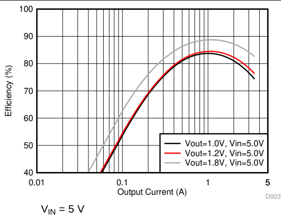
Figure 85. Buck Efficiency in Forced PWM Mode
