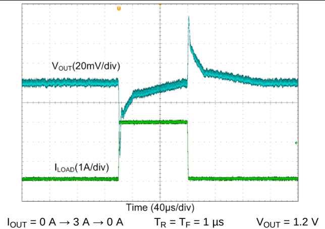
Figure 98. Buck Transient Load Step Response, Forced-PWM Mode
