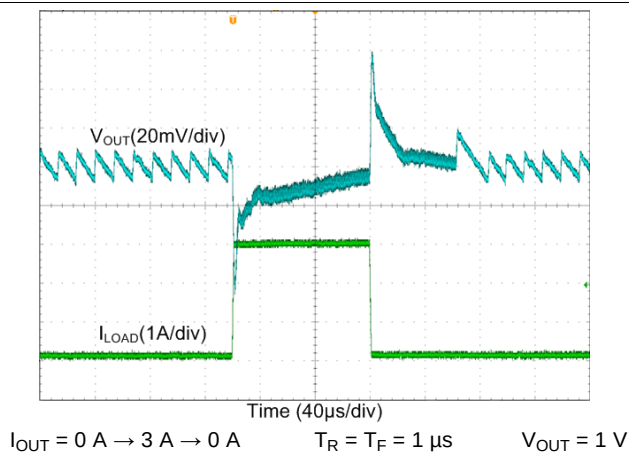
Figure 99. Buck Transient Load Step Response, Auto Mode
