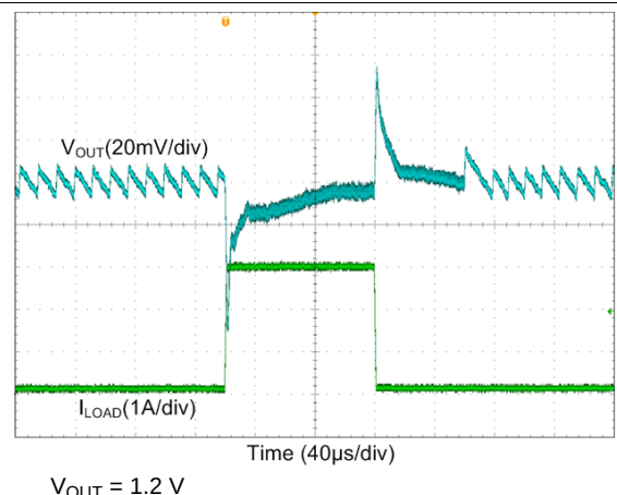
Figure 100. Buck Transient Load Step Response, Auto Mode
