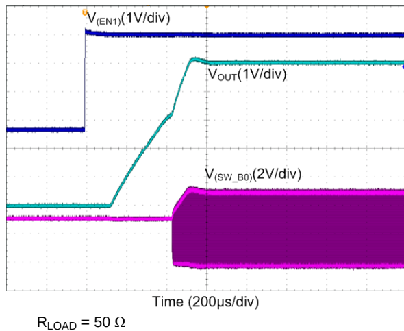
Figure 105. Boost Start-up With EN1, Forced-PWM
