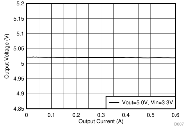
Figure 102. Boost Output Voltage vs Load Current
