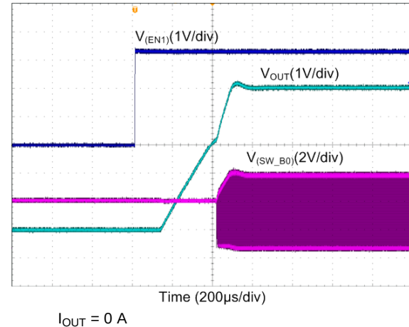
Figure 104. Boost Start-up With EN1, Forced-PWM
