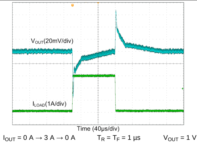
Figure 97. Buck Transient Load Step Response, Forced-PWM Mode
