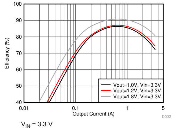
Figure 84. Buck Efficiency in Forced PWM Mode
