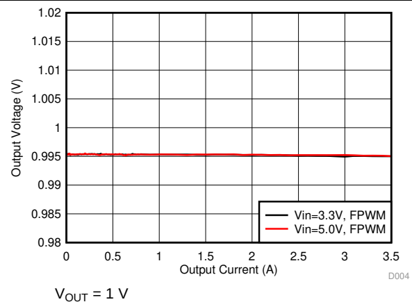
Figure 86. Buck Output Voltage vs Load Current in Forced PWM Mode
