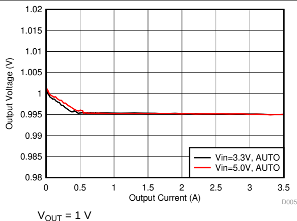
Figure 87. Buck Output Voltage vs Load Current in AUTO Mode
