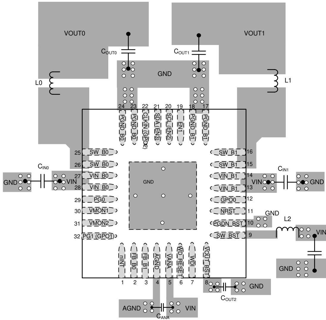
Figure 109. LP87702-Q1 Board Layout Example
