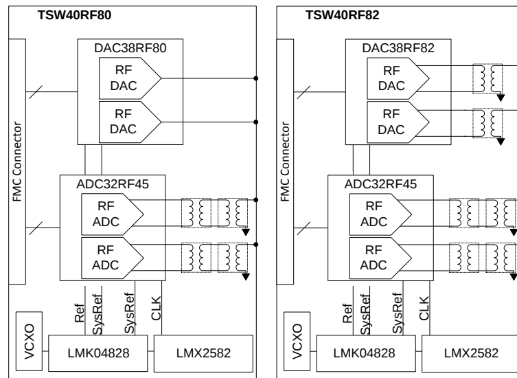
Figure 1. EVM Block Diagram
