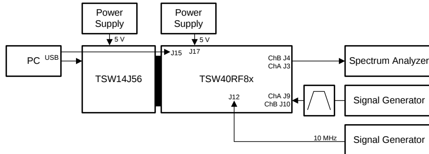
Figure 2. Test Set-Up Block Diagram
