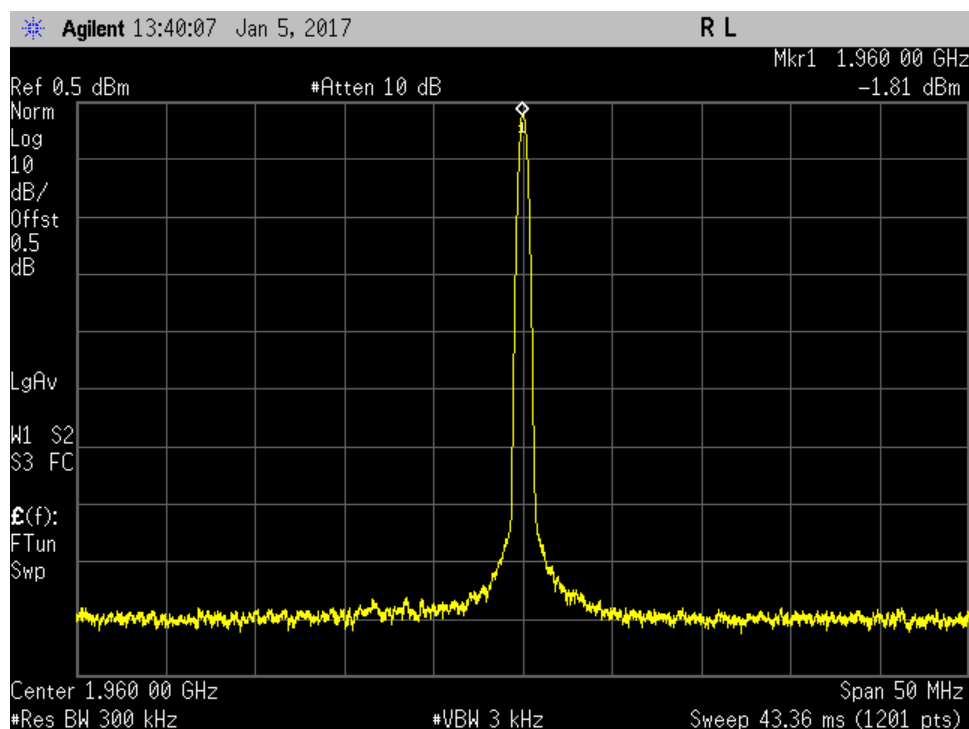
Figure 3. DAC Output Spectrum
