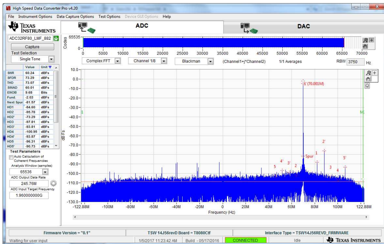
Figure 4. Captured Output Tone
