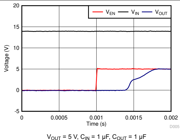
Figure 6-18. Startup With Enable
