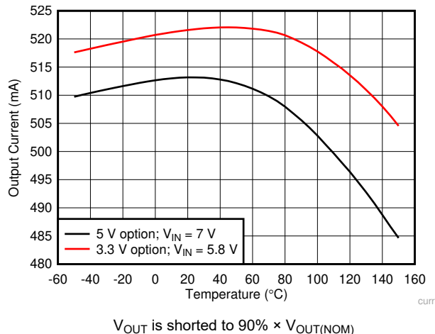
Figure 6-14. Output Current Limit vs Ambient Temperature
