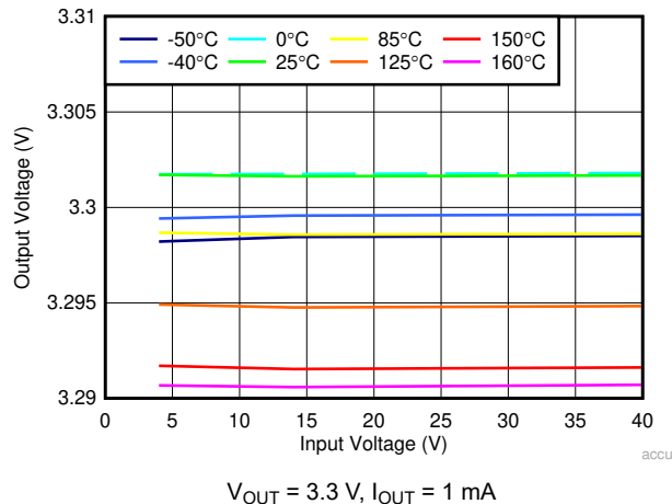
Figure 6-13. Output Voltage vs Input Voltage
