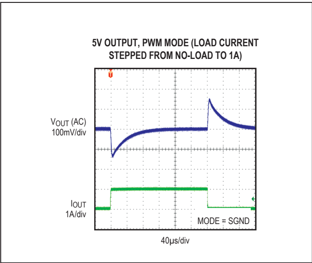
Figure 7. MAX17543 5V Output, No Load to 1A Load Transient (PWM Mode)
