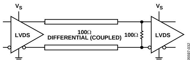
Figure 38. LVDS Output Termination
