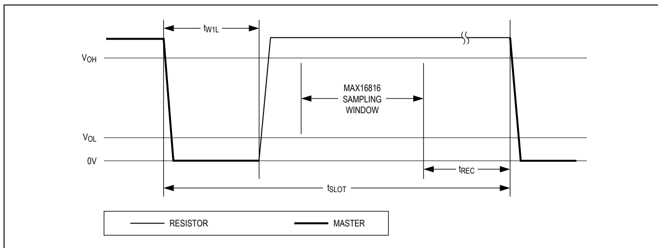
Figure 7. 1-Wire Write-1 Time Slot
