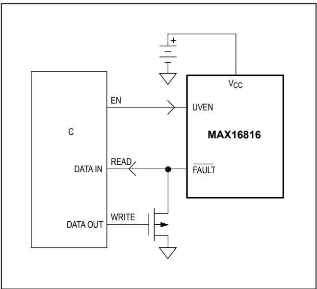
Figure 5. Programming Through a \overline{\text{FAULT}} Pin
