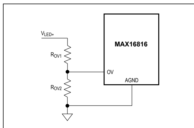
Figure 4. Setting the Overvoltage Threshold
