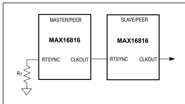
Figure 3. Master-Slave/Peer-Peer Clock Configuration
