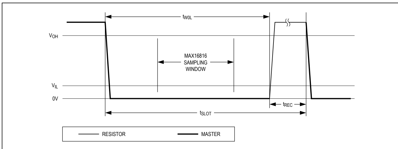
Figure 8. 1-Wire Write-0 Time Slot
