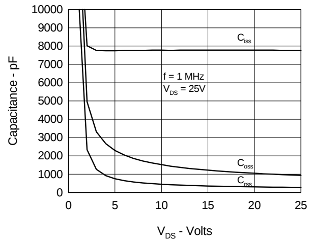
Fig.8 Capacitance Curves
