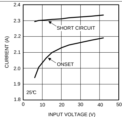
Figure 30. Current Limit 3.3 V_{OUT} at 25^\circ\text{C}
