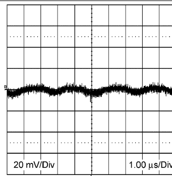
Figure 26. Output Ripple 24- V_{IN} 3.3- V_O 1-A, BW = 200 MHz
