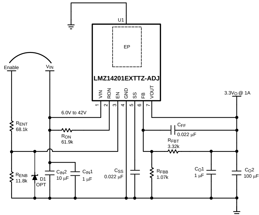
Figure 34. Evaluation Board Schematic Diagram
