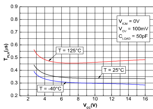
Figure 15: Propagation delay t_{PLH} vs. supply voltage
